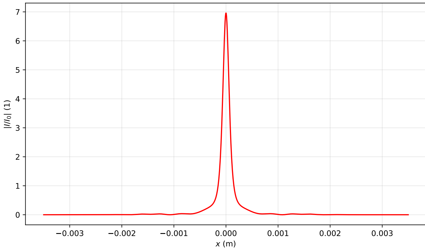
Intensity profile I(x, y = 0, z = 1.911)/I_0 , P_{in}=4.0P_{cr} , artificial time
